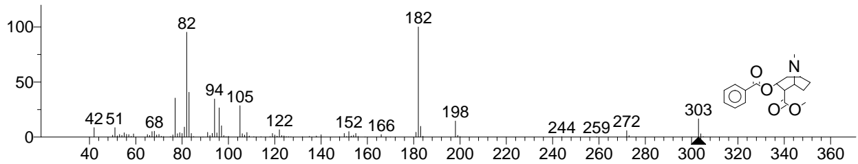
(replib) Allopseudococaine
